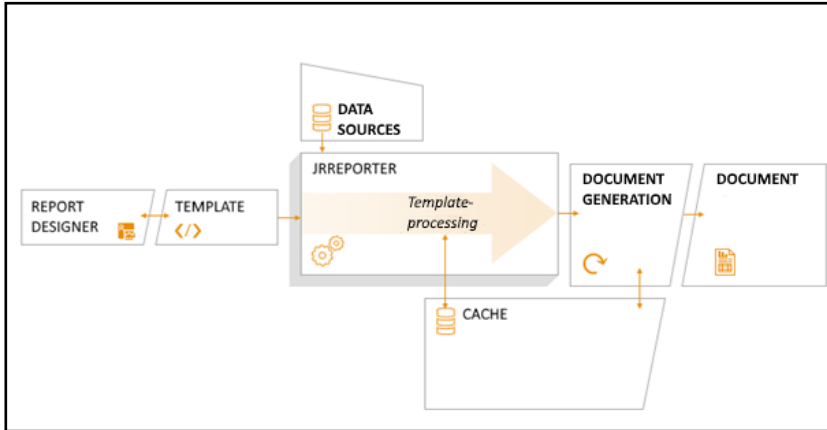
Schematic functionality of the JRReporter
